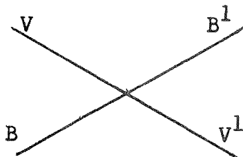
The Motional Electric and Magnetic Fields of Hooper
